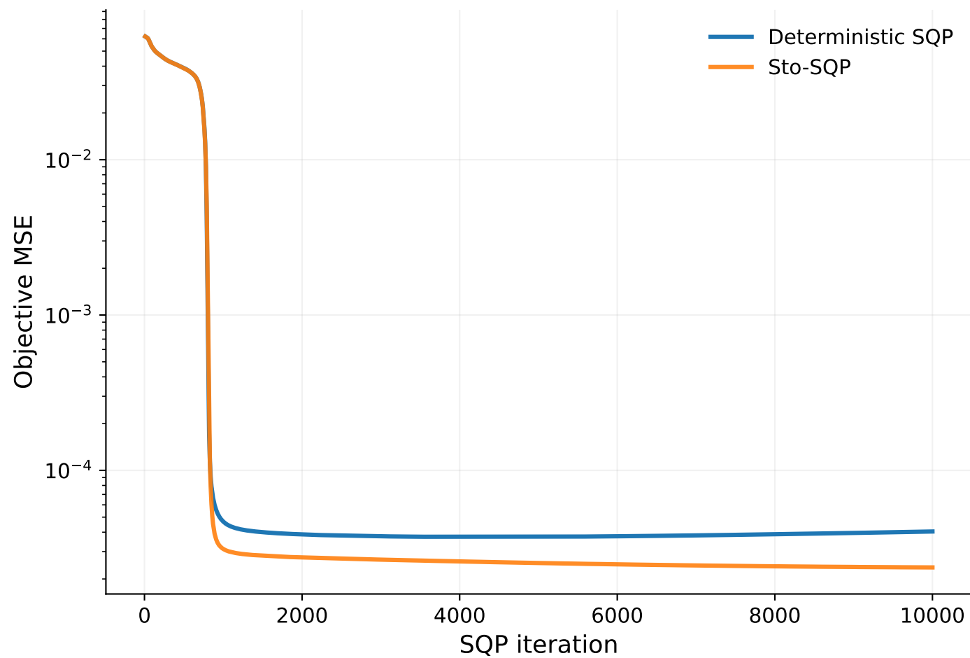
Allen-Cahn equation: objective MSE
